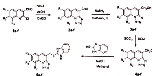
Scheme-1: Synthesis of 4-((1H-benzo[d]imidazol-2-ylthio)methyl)tetrazolo[1,5-a]quinolines derivatives
