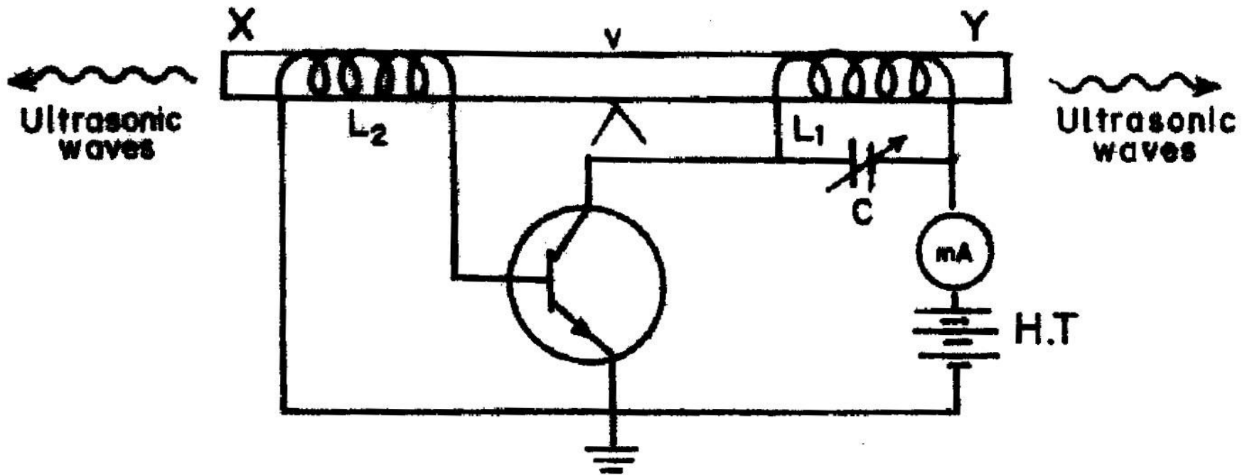
Magnetostriction oscillator
